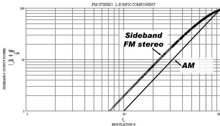
FIG 11 FM stereo sidebands at 38 kHz sub carrier
