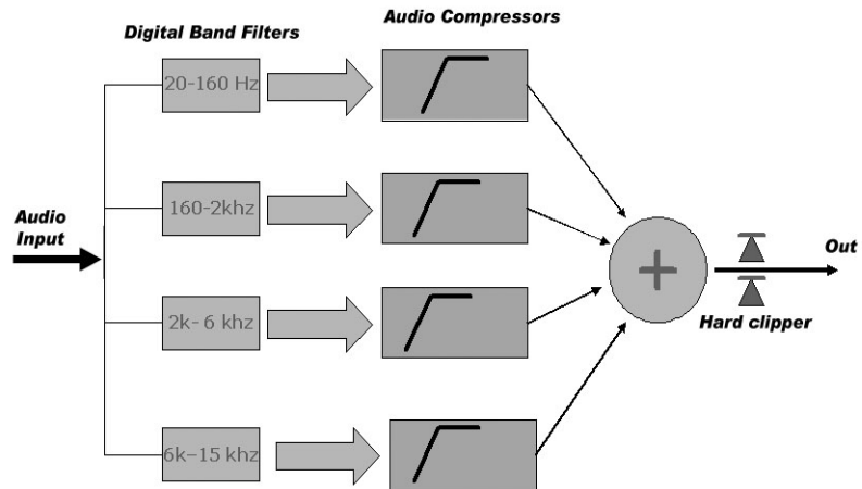
FIG 1 Block Diagram of multiband compressor
