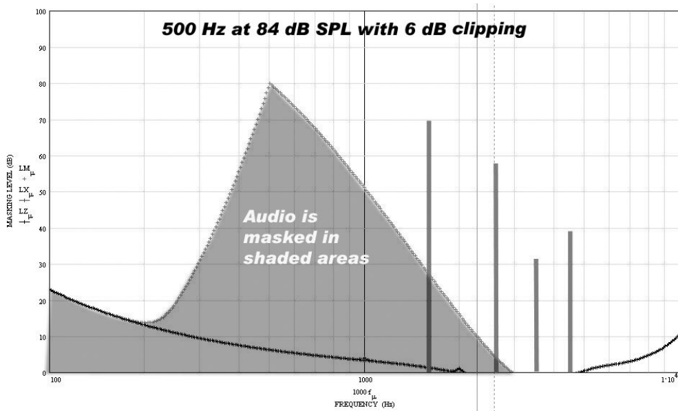
FIG 4 Harmonics of the 500 Hz clipped wave
