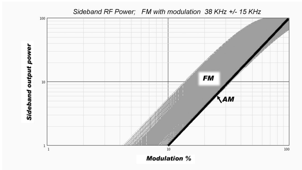
FIG 12 FM stereo with MPX modulation 30-15.000 Hz
