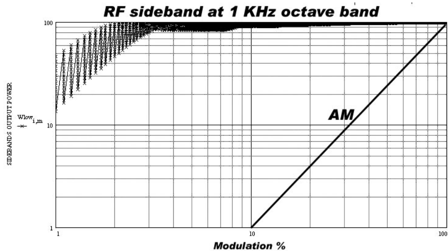
FIG 9 FM modulation sidebands at 1 kHz octave band (707-1414 Hz) for 100 W FM transmitter, compared with a 200 W AM transmitter.
