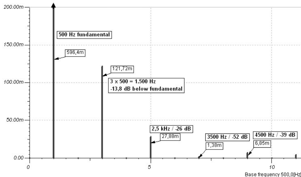
FIG 3 500 Hz, 6 dB clipping, harmonic spectrum
