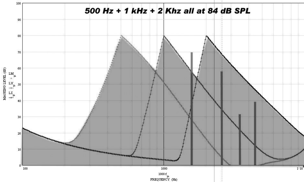
FIG 6 Masking 500 Hz clip, with 3 bands, at the same level
