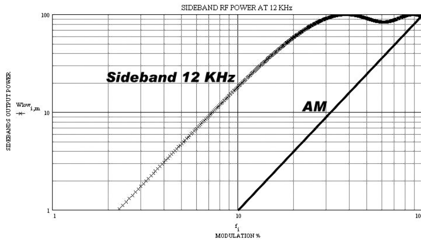
FIG 10 FM sidebands at 12 kHz modulation
