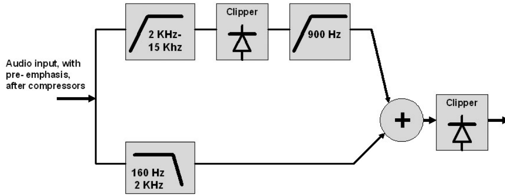
FIG 8 Dual bands IM cancelled clipper
